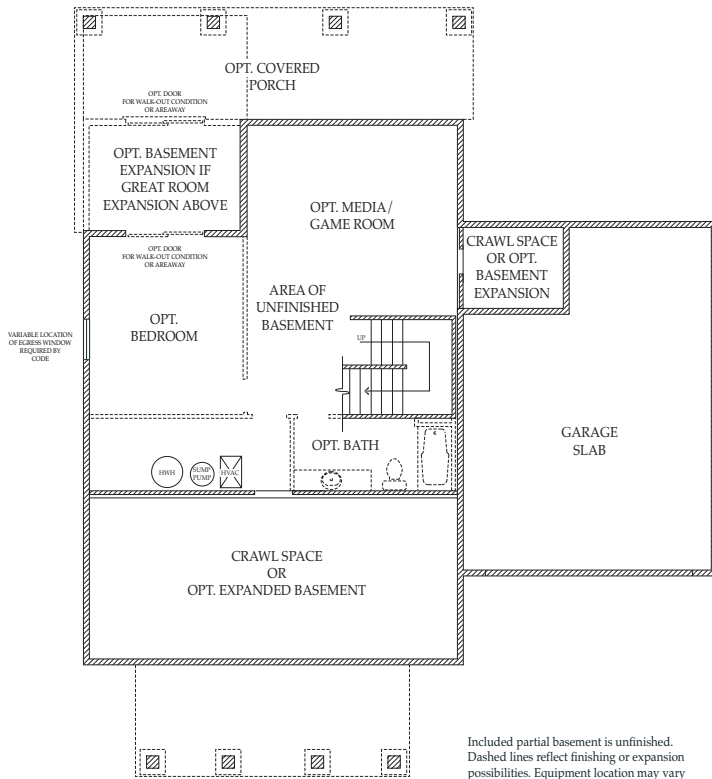
LOWER LEVEL FLOOR PLAN Partial Unfinished Basement Showing Optional Media/Game Room, Bedroom or Areas for Basement Expansion
