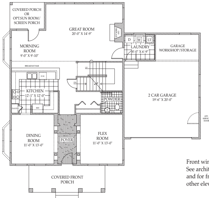
MAIN LEVEL FLOOR PLAN
