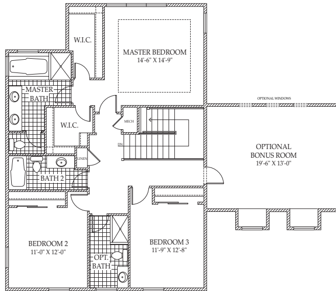
UPPER LEVEL FLOOR PLAN with Bonus Room Option and Bath Option over Entry
