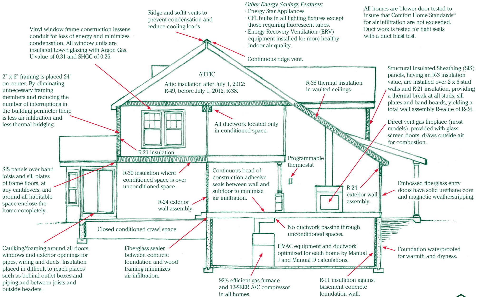
Representational cross section through home is without reference to model type.
